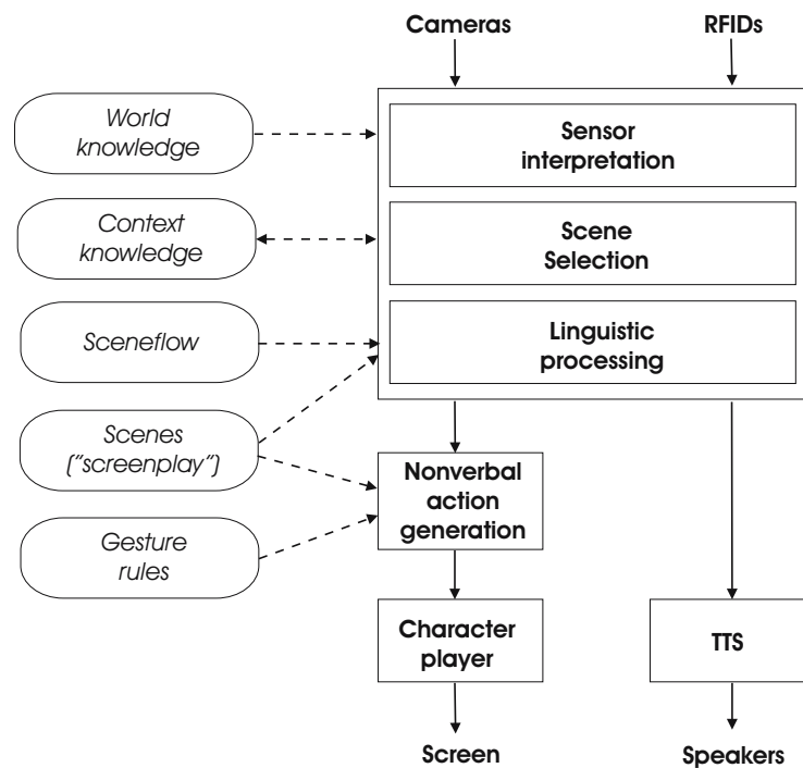
Fig. 2. Overview of the COHIBIT runtime system architecture
